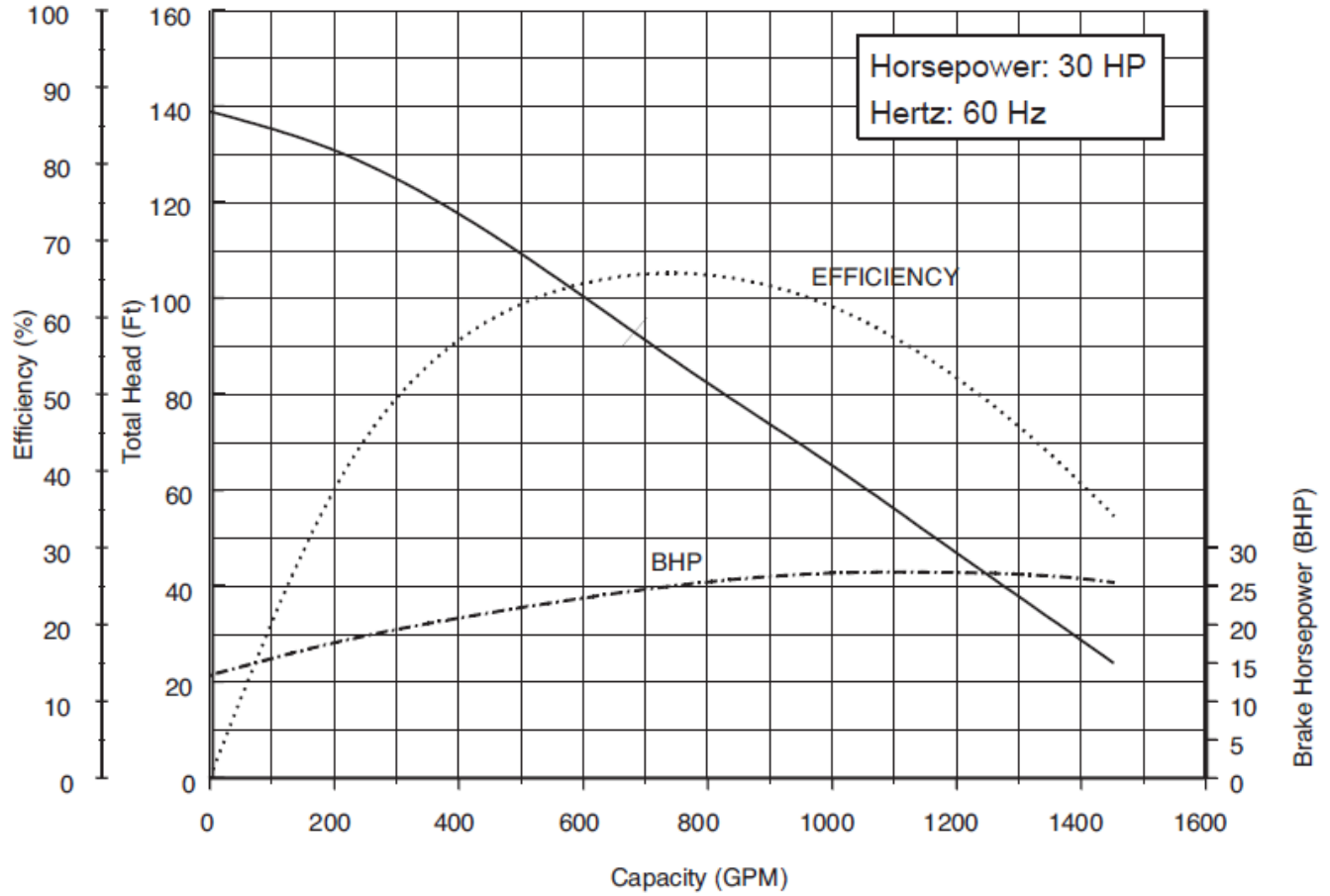
Stancor Model 100LX622 Individual Performance Curve
