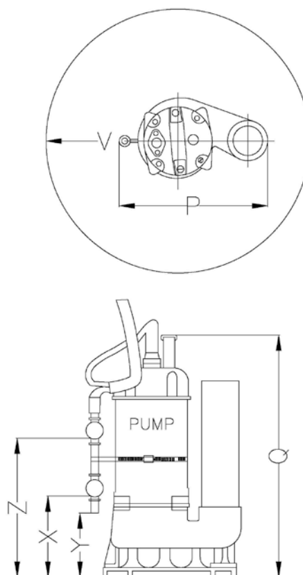
Installation Dimensions
