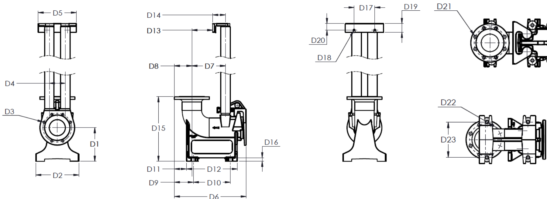
Dimensions in mm unless otherwise specified
